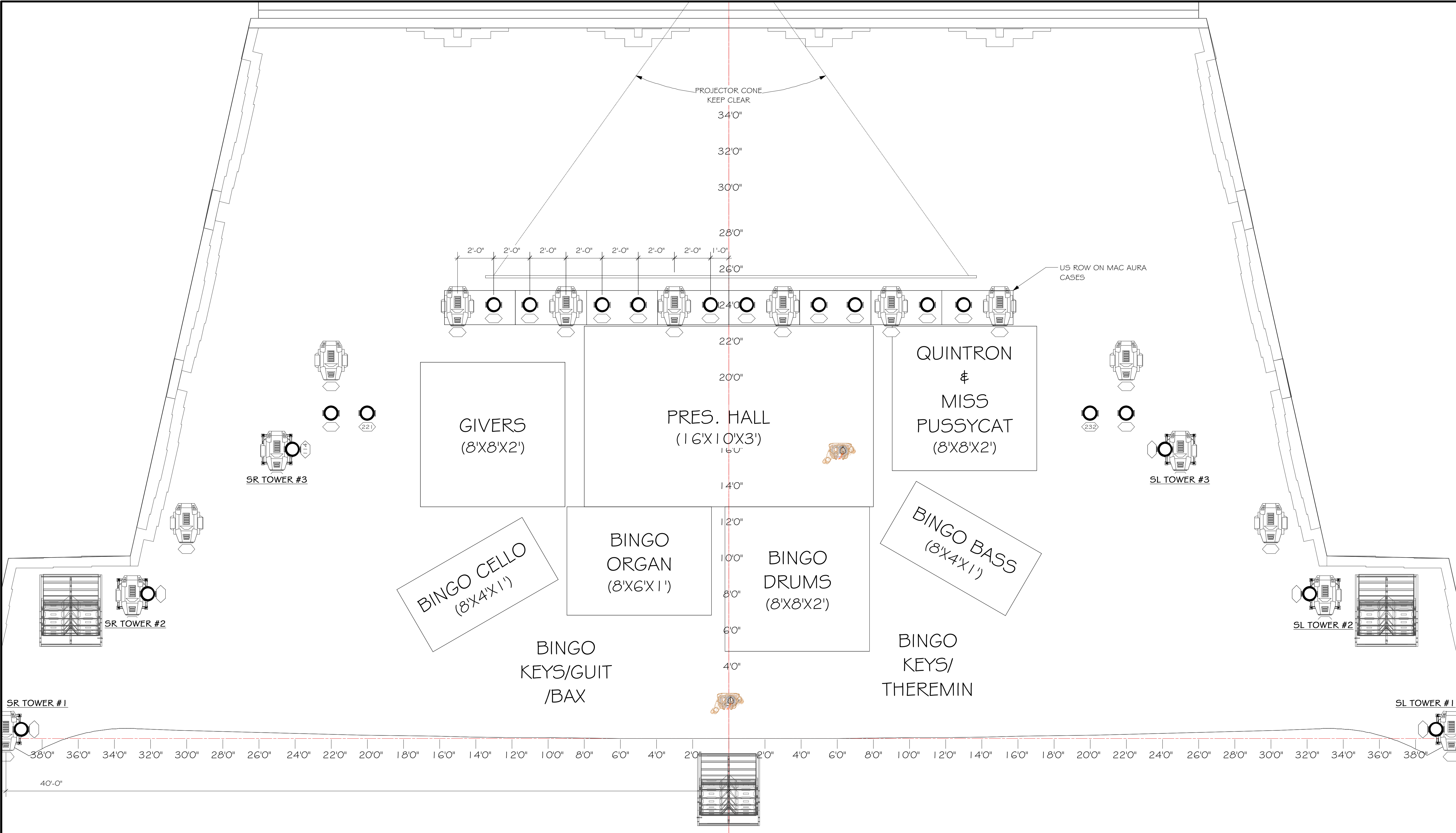
1 DECK FIXTURE PLOT 3/8" = 1'0"
